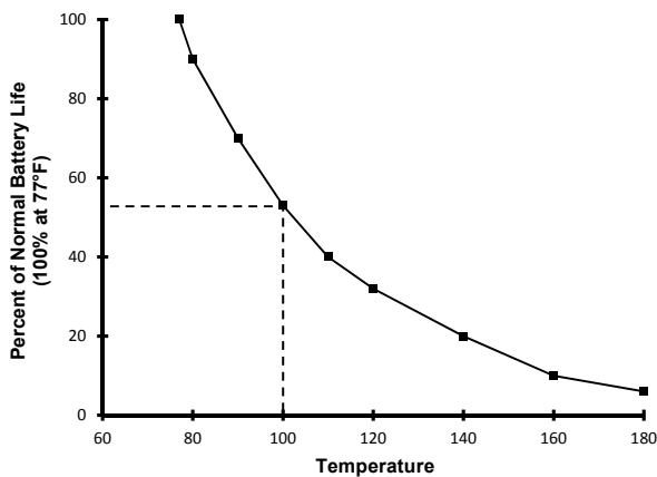
FIGURE 3 - Temperature vs. Battery Life Curve
